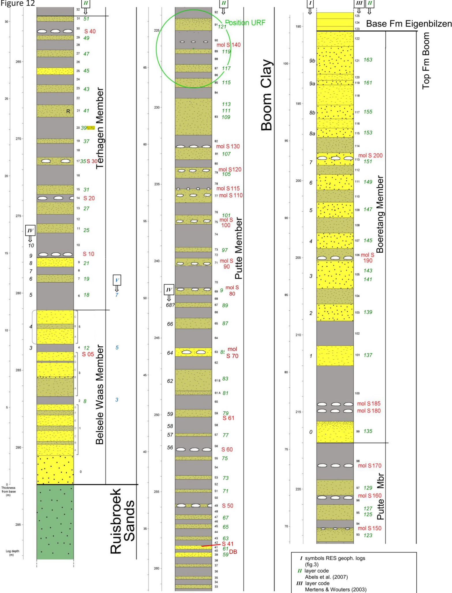
Microstratigraphic litholog of the Boom Formation based on the FMI (Full bore Formation Micro Imager) of the boreholes ON-Mol-1 en ON-Dessel-1 (Mertens & Wouters, 2003). The existing numbering systems of the layers (Abels et al., 2007; Vandenberghe, 1978; Van Simaey, 2004) are plotted in several columns in parallel to the layer codes introduced by Mertens & Wouters (2003) for their litholog.
