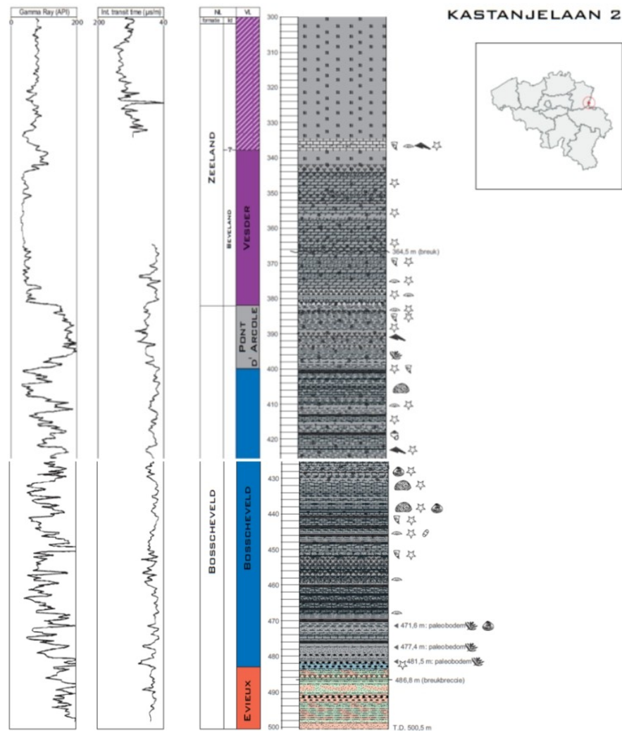
Figure 8. Litholog of Lower Carboniferous and Devonian sequence of borehole Kastanjelaan-2, stratotype for the Bosscheveld Formation. (From Laenen, 2003)
