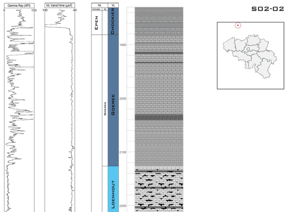
Figure 7. Litholog of Lower Carboniferous and Devonian sequence of borehole S02-02, stratotype for the Goeree Formation. (From Laenen, 2003)
