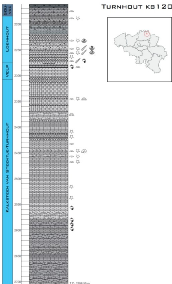
Figure 6. Litholog of Lower Carboniferous and Devonian sequence of borehole 017E225 (KB120, Turnhout, Zwemdok), stratotype for the Steentje-Turnhout Formation. (from Laenen, 2003)
